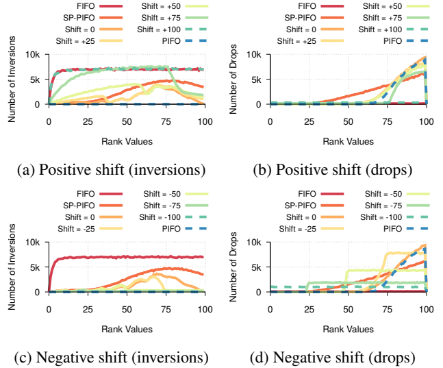
Figure 11: Rank-distribution sensitivity (TCP uniform).
