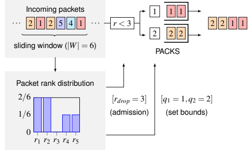
Figure 5: PACKS closely approximates PIFO’s behavior.
