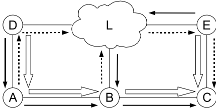
Figure 1: Sample network. Bold arrows mark the shortest path to C , dashed arrows mark the primary and solid arrows mark the secondary redundant tree rooted at C .
