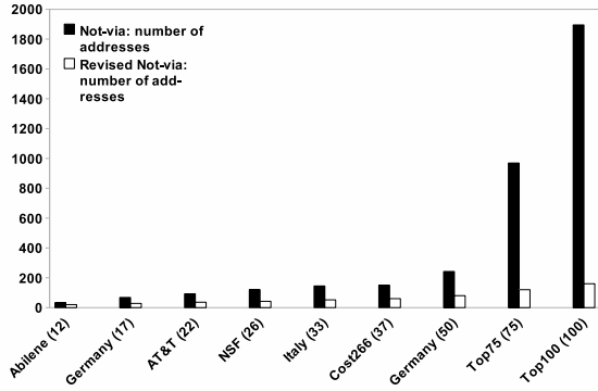
Figure 3: Number of additional addresses for the original and lightweight Not-via in commonplace ISP topologies (number of nodes is given in parentheses), with every fifth node substituted by a LAN.
