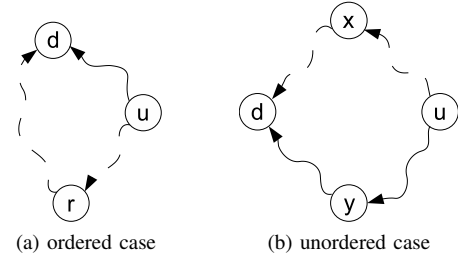
Figure 2: Illustration for Theorem 1.
