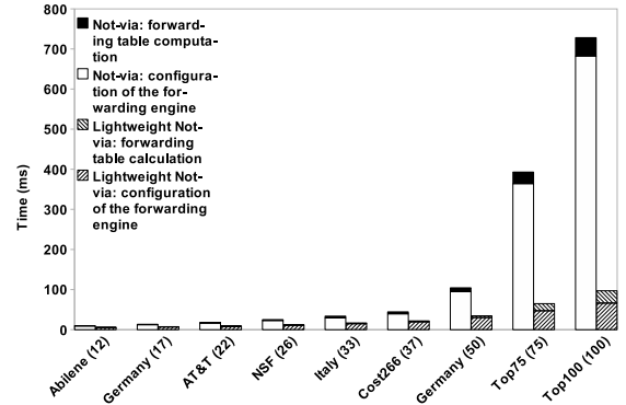
Figure 4: Execution time of computing the default and backup next-hops and configuring the forwarding engine for the original and the lightweight Not-via.
