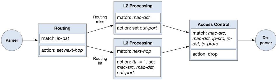
Fig. 4. Simplified match-action table dependency graph for a basic router (inspired by Fig. 3 in Reference [22]).
