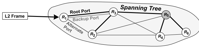
Fig. 9. Illustration of the example configuration of a spanning tree for RSTP rooted at node R_5 : An incoming frame is forwarded by R_1 by default in the direction of the root node ( R_5 here) via the respective Root Port outgoing from R_1 towards R_3 . In the case of a failure of the primary link R_1 – R_3 , the frame can be forwarded along a duplicate link via the Backup Port . However if both direct links between R_1 and R_3 are not available (e.g., due to their failure), the frame can be forwarded via the Alternate Port towards node R_2 .
