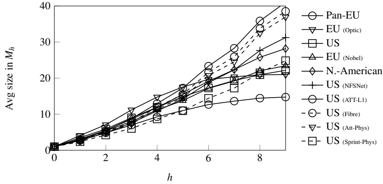
Fig. 1.2 The average number of links contained in the SRLGs of M_h in case of physical backbone topologies of [25]
