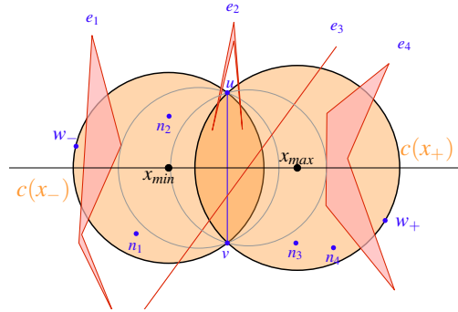
Fig. 1.3 Illustration of an apple with k = 2 . Apple A_k^{u,v} consists of specific ordered lists of links and nodes which can be hit by a disk from C_k^{u,v} . For more details, please check [38]
