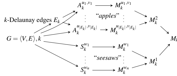
Fig. 1.4 Sketch of algorithm from [38] for enumerating set M_k of maximal link sets which can be hit by a circular disk hitting k nodes
