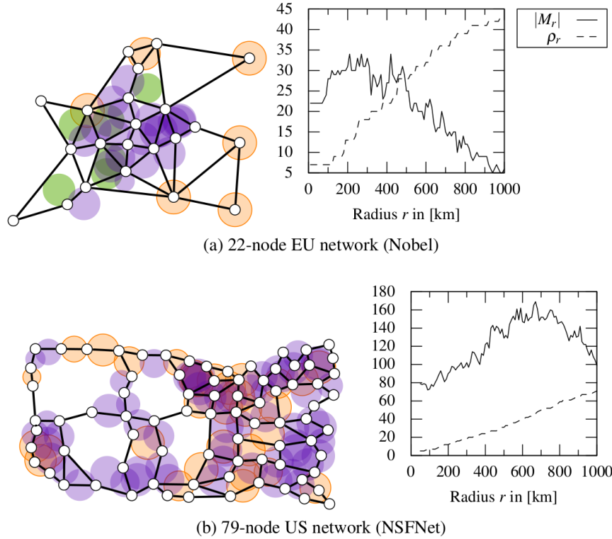
Fig. 1.7 Simulation results for determining list M_r of maximal SRLGs of disasters being circular disks with radius r
